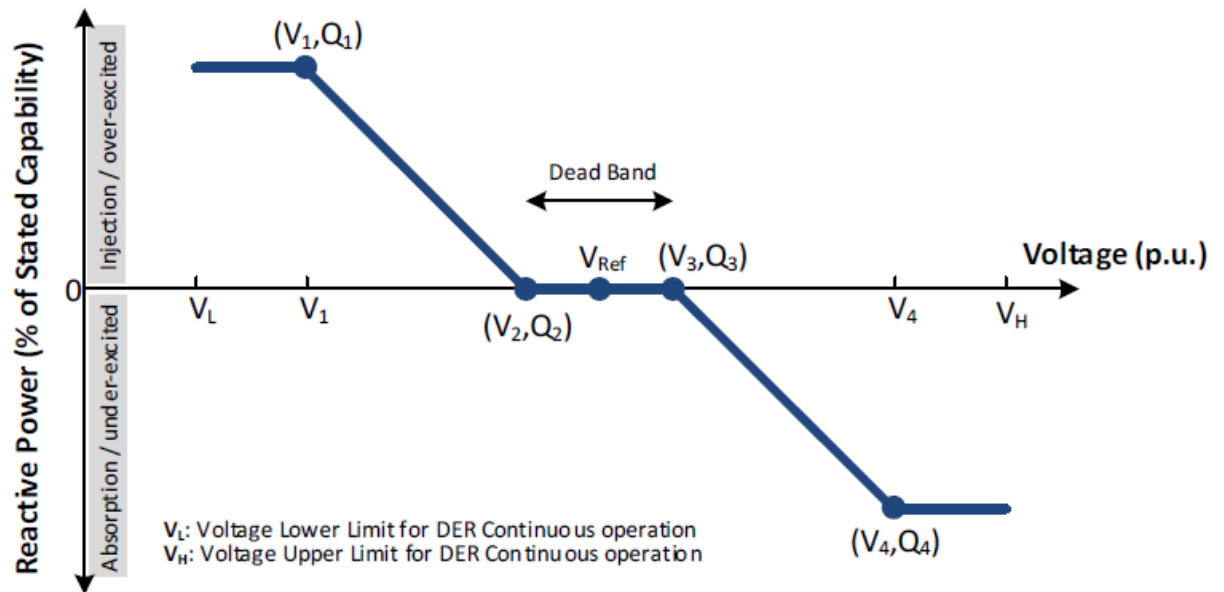
Figure H.4—Example voltage-reactive power characteristic
