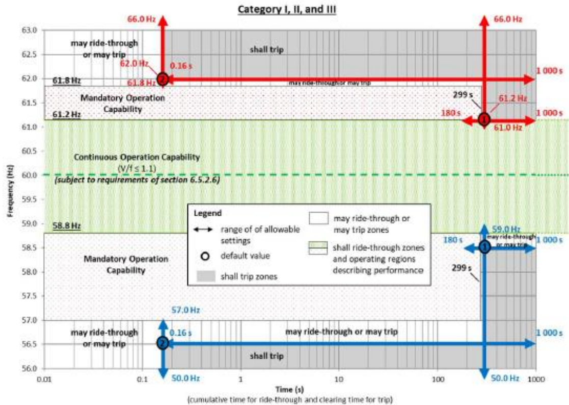
Figure 5: DER default response to abnormal frequencies and frequency ride-through requirements for DER of abnormal operating performance Category I, II, and III
